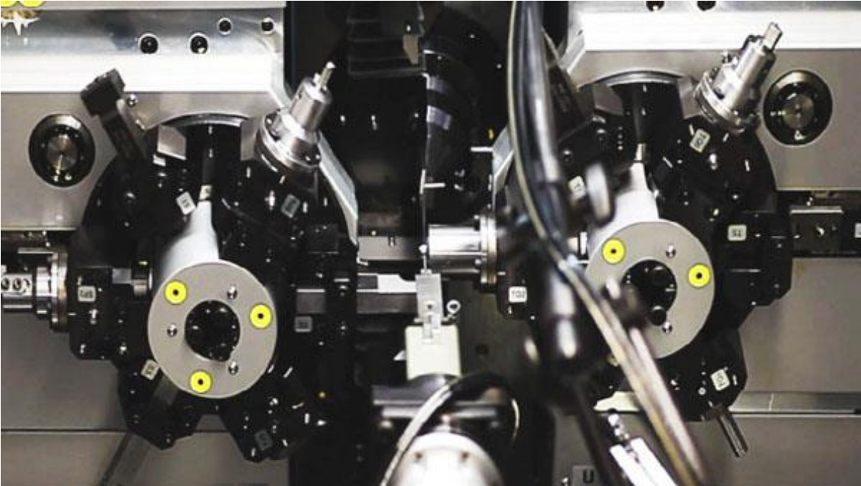
Picture 4: wire bending process
